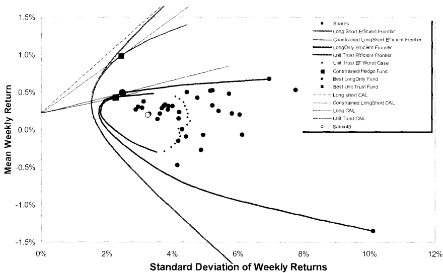
Figure 1: The risk-return map using weekly data from the ALSI 40 constituents from December 2000 to September 2004. The post-hoc optimal portfolios and efficient frontiers are shown for unconstrained long-short, constrained long-short, long (only), unit trust portfolios.
