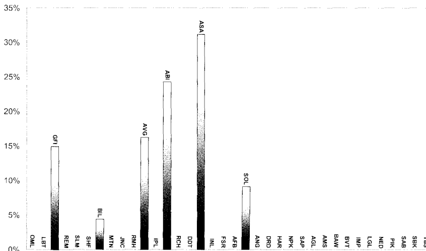
Figure 2: Long only constituents – no constraints. The optimal long-only portfolio consists of only six equities, and with more than 30% in Absa.
